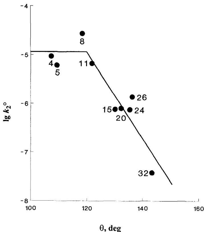
Fig. 2. The steric profile [22] for reactions of (\eta^5\text{-Me}_5\text{C}_5)\text{Rh}(\text{CO})_2 with P-donor nucleophiles in toluene (standard reactivity, -4.9 \pm 0.03 ; \theta_{\text{th}} = 120^\circ ; \beta = 0.09 \pm 0.05 , \gamma = -0.093 \pm 0.017 \text{ deg}^{-1} ; r.m.s. deviation, 0.30).
