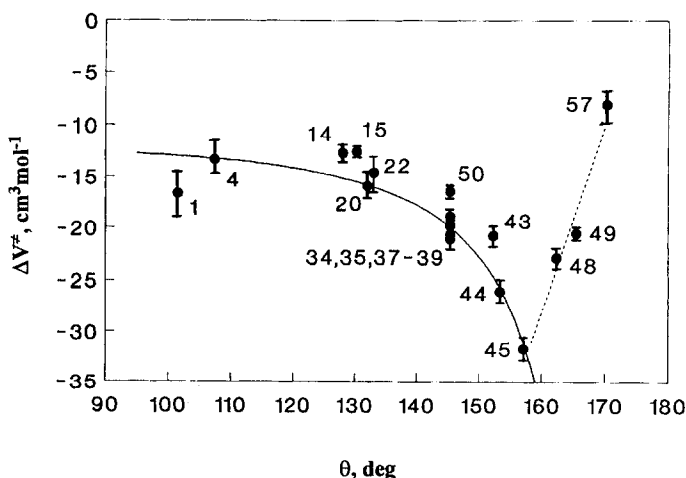
Fig. 8. Correlation of values of \Delta V^\ddagger and \theta for reactions of (\mu\text{-H})_2\text{Os}_3(\text{CO})_{10} with L in chlorobenzene to form (\mu\text{-H})(\text{H})\text{Os}_3(\text{CO})_{10}\text{L} . The full curve is drawn according to Eq. (11).
